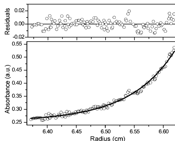
Figure 4. AUC equilibrium experiment of 0.10 \mu M anti-DNP IgG incubated with 0.067 \mu M 1 at 6 K rpm as observed at 230 nm at 25 °C. The hollow circles are experimental data, and the line is the fit for a single ideal species. The expected molecular mass is \sim 450 \pm 12 kDa, and the calculated molecular mass is 464 \pm 35 kDa.
